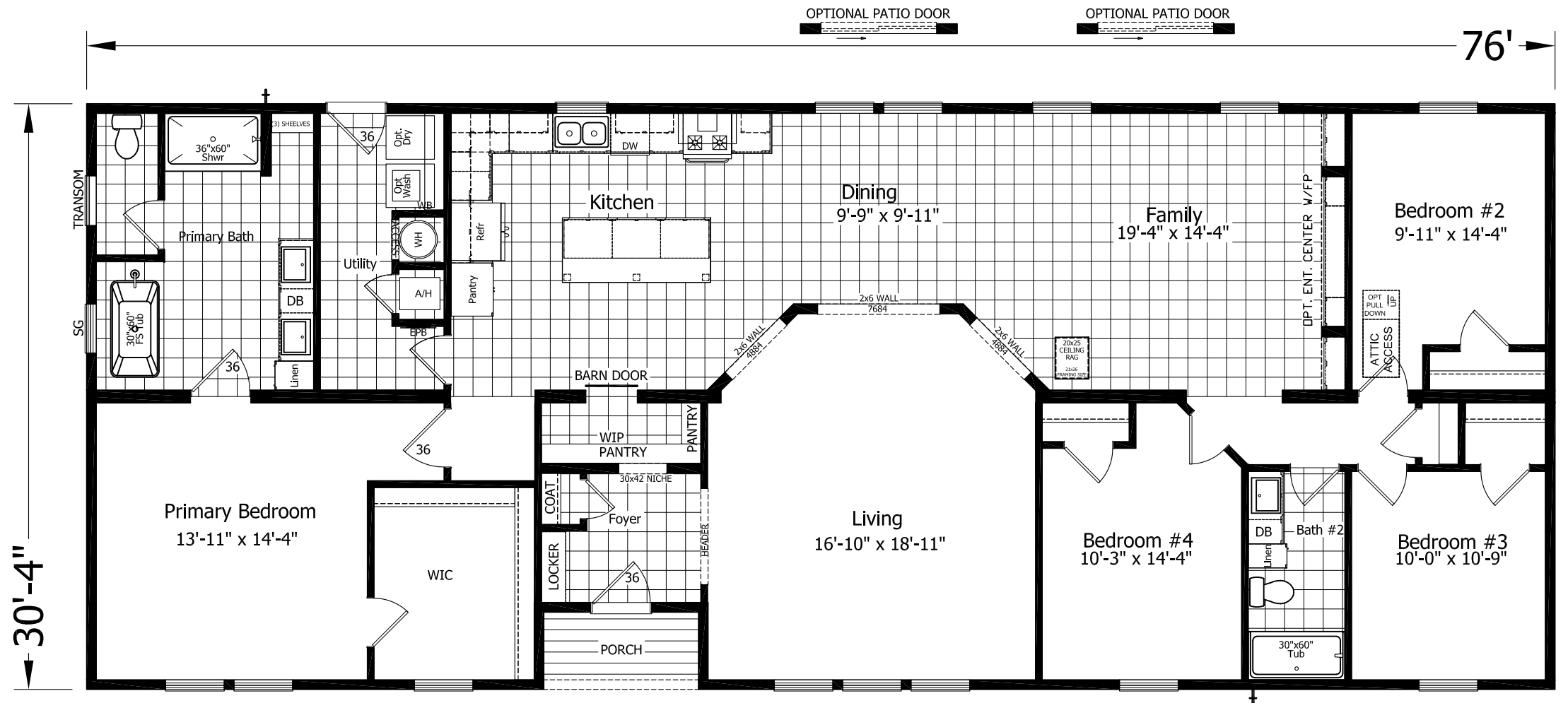
70-3276-05 TRYON 4 Bedroom 2 Bath 76'-0" x 30'-4" 2273 Sq. Ft. Total
